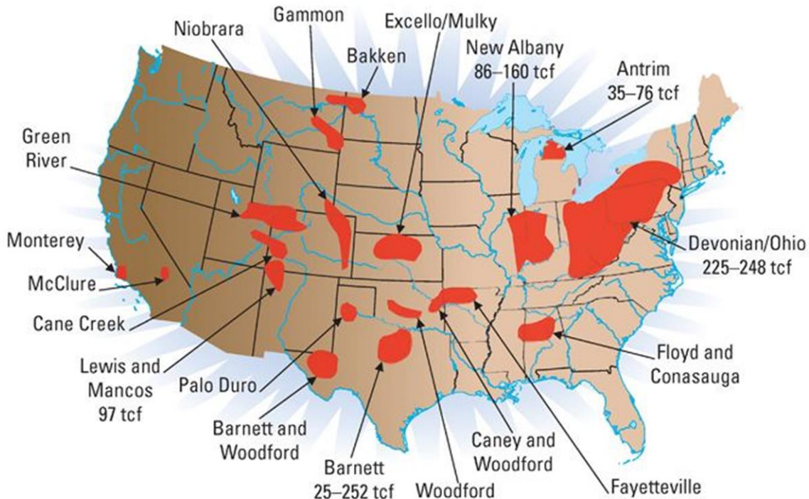
Major shale gas basins in the United States with total resource potential of 500 to 1,000 trillion cubic feet (tcf). Map courtesy of Schlumberger.
